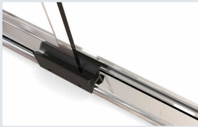
Stay-Kleen track & guide, bypass enclosures
