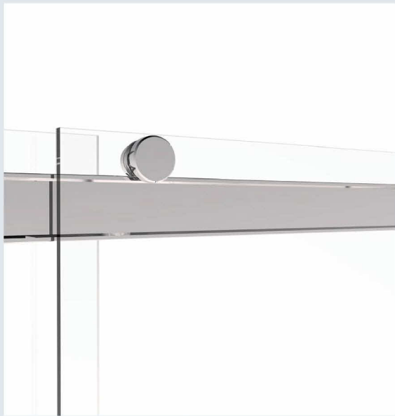
Header with visible top rollers, bypass enclosures
