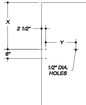
DOOR GLASS DETAIL HINGE RIGHT SHOWN REVERSE FOR HINGE LEFT
