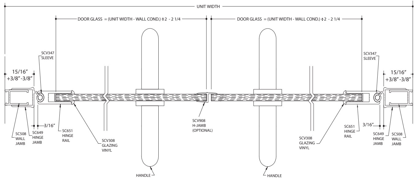
HORIZONTAL CROSS SECTION
