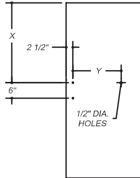
DOOR GLASS DETAIL HINGE RIGHT SHOWN REVERSE FOR HINGE LEFT
