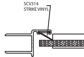
STRIKE JAMB DETAIL ABOVE & BELOW MAGNET
